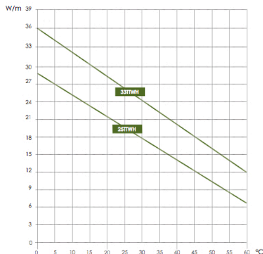
CURVA TERMICA TEMPERATURE CURVE
